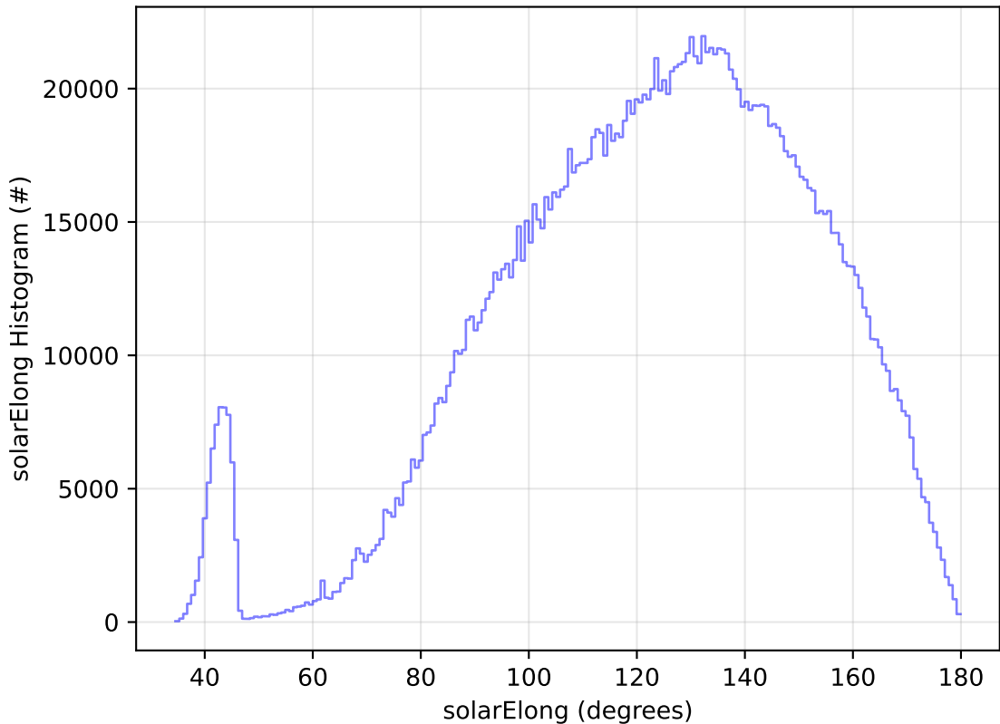
early_u_fpextra3.0_v3.4_10yrs All sky all bands: solarElong Histogram
