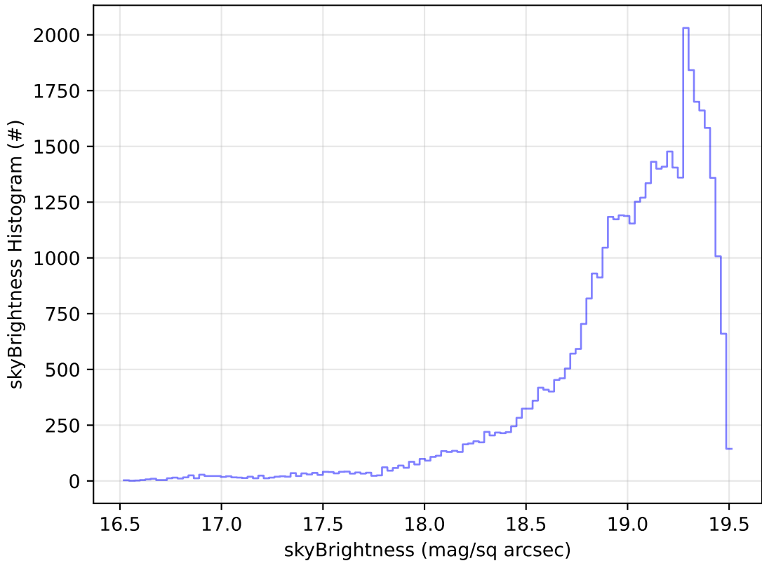
early_u_fpextra3.0_v3.4_10yrs Yr 1 z band: skyBrightness Histogram
