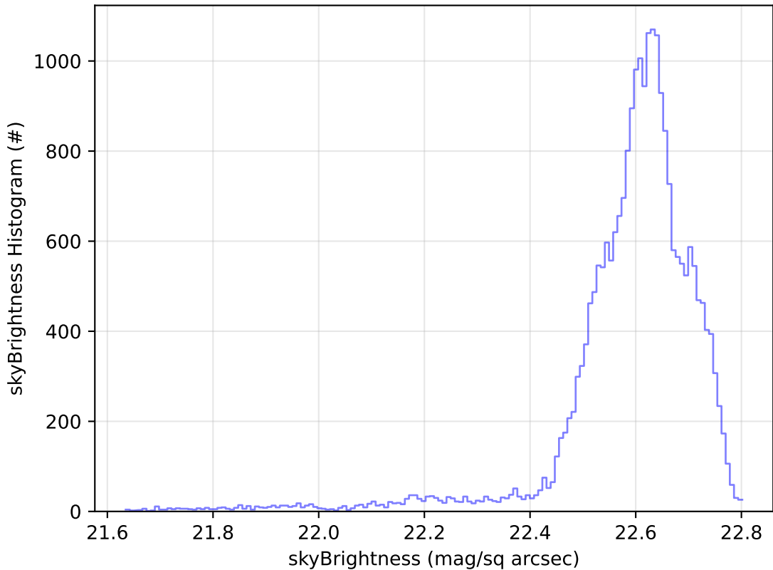
early_u_fpextra3.0_v3.4_10yrs Yr 1 u band: skyBrightness Histogram
