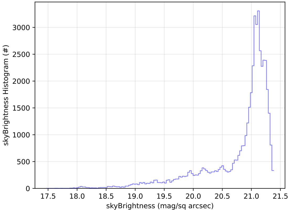
early_u_fpextra3.0_v3.4_10yrs Yr 1 r band: skyBrightness Histogram
