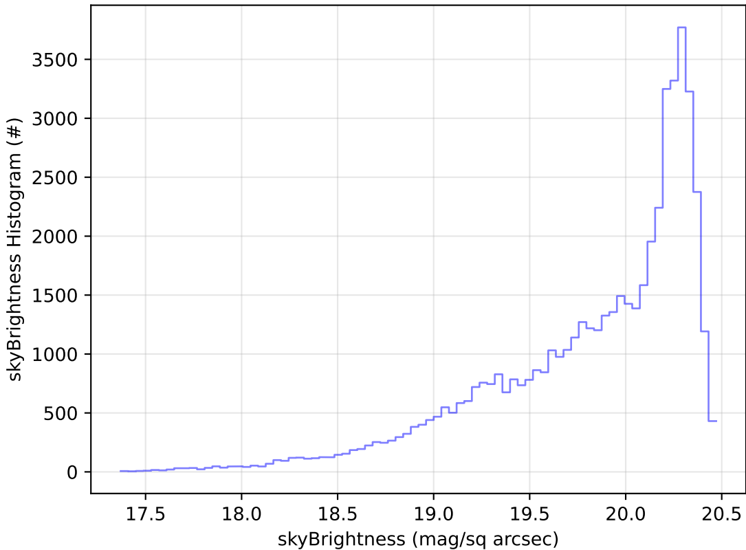
early_u_fpextra3.0_v3.4_10yrs Yr 1 i band: skyBrightness Histogram
