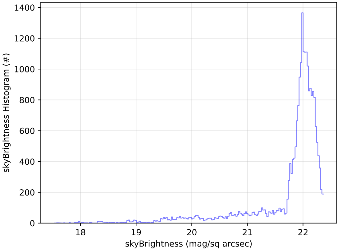
early_u_fpextra3.0_v3.4_10yrs Yr 1 g band: skyBrightness Histogram
