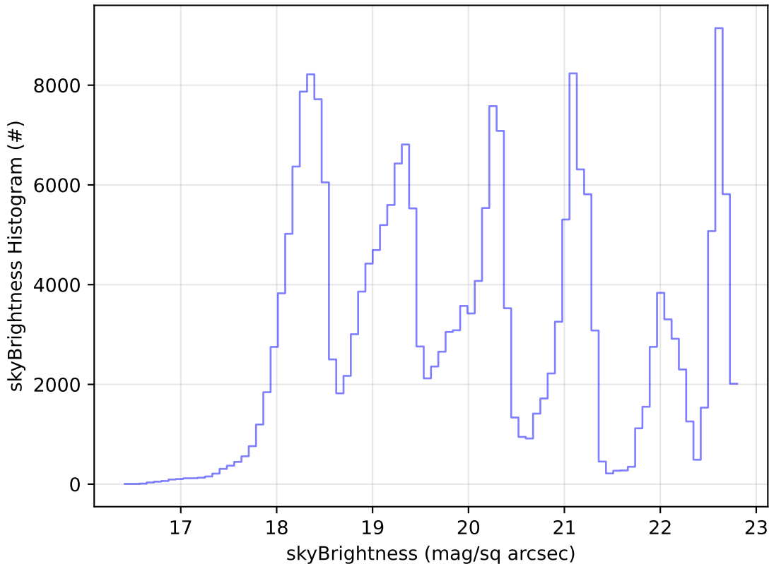
early_u_fpextra3.0_v3.4_10yrs Yr 1 all bands: skyBrightness Histogram
