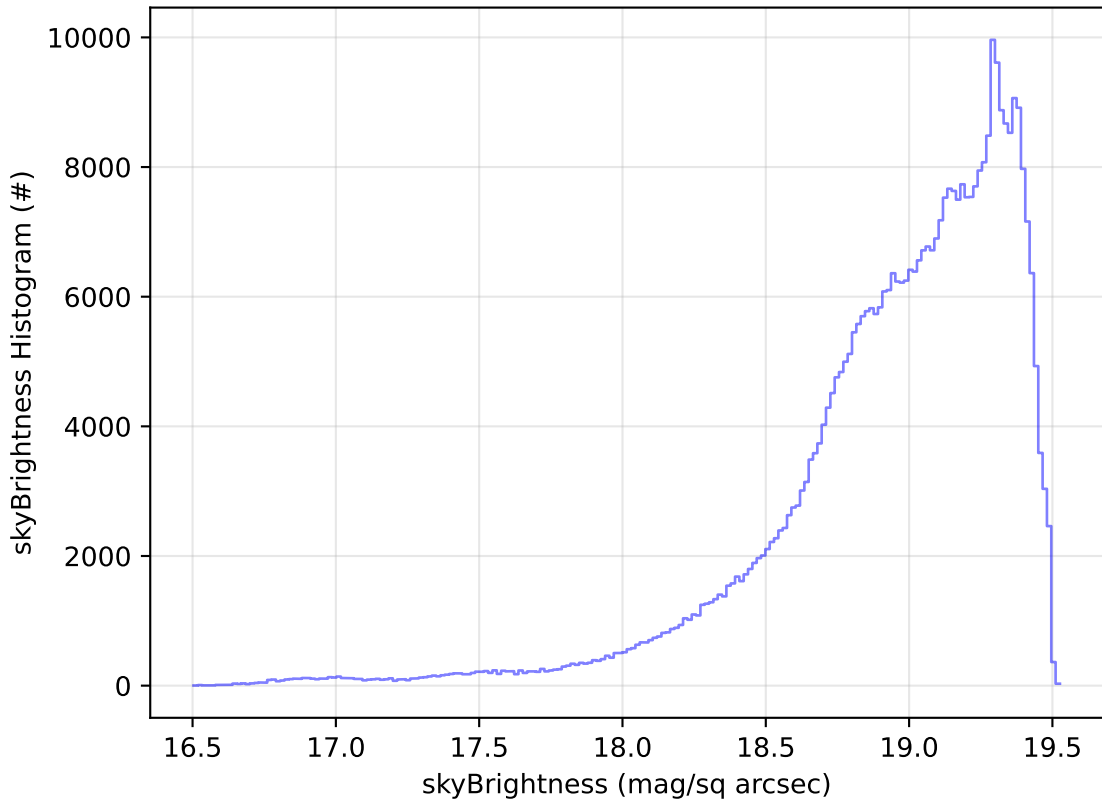
early_u_fpextra3.0_v3.4_10yrs WFD z band: skyBrightness Histogram
