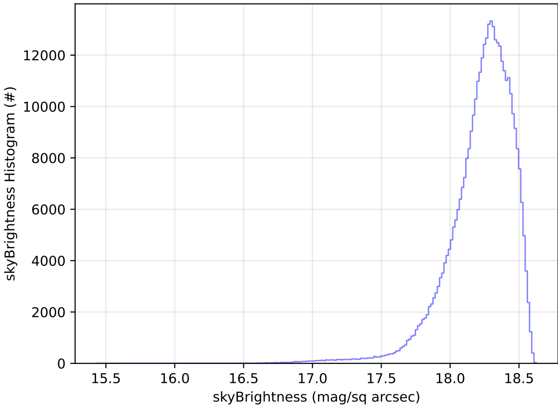
early_u_fpextra3.0_v3.4_10yrs WFD y band: skyBrightness Histogram
