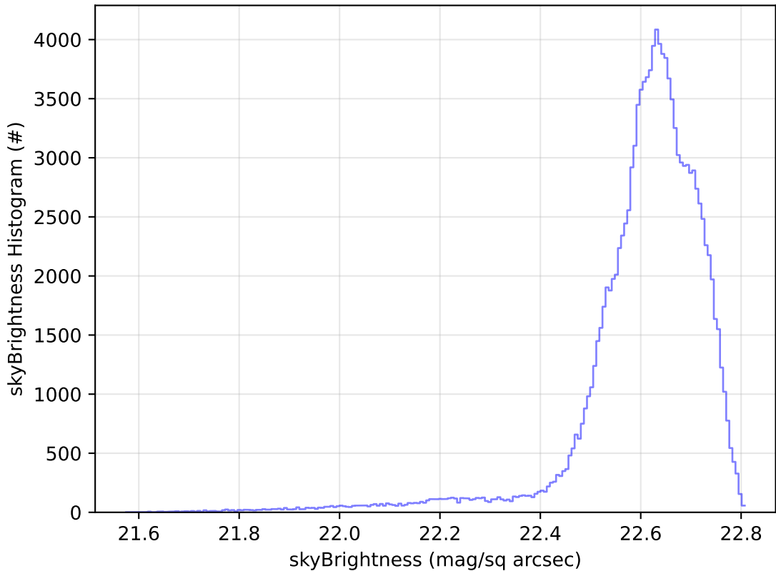
early_u_fpextra3.0_v3.4_10yrs WFD u band: skyBrightness Histogram
