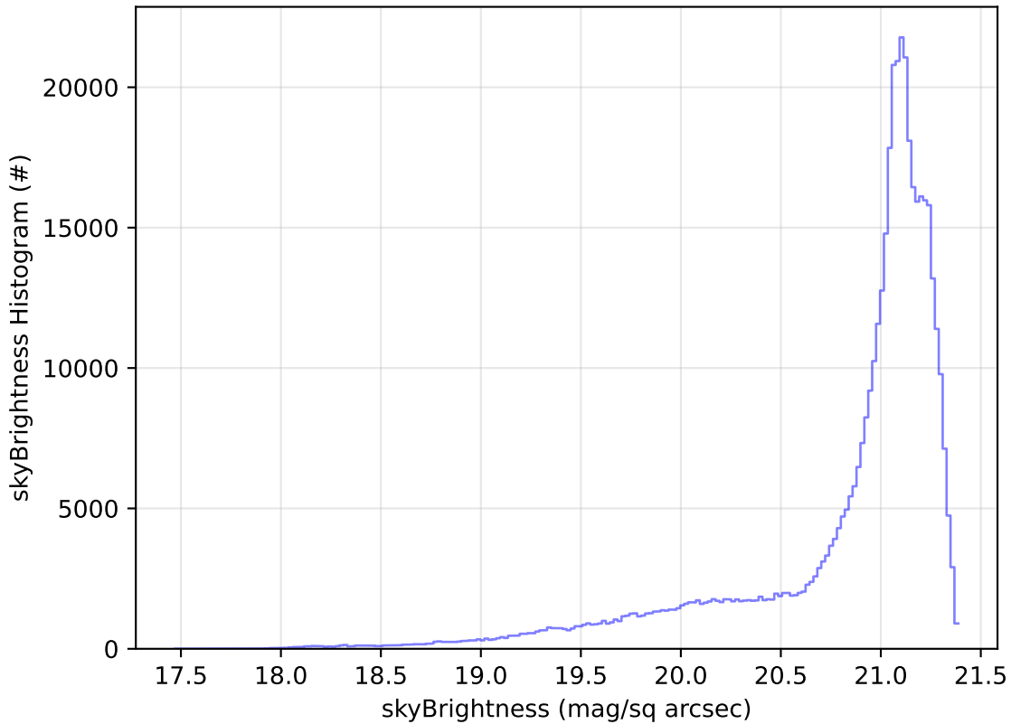
early_u_fpextra3.0_v3.4_10yrs WFD r band: skyBrightness Histogram
