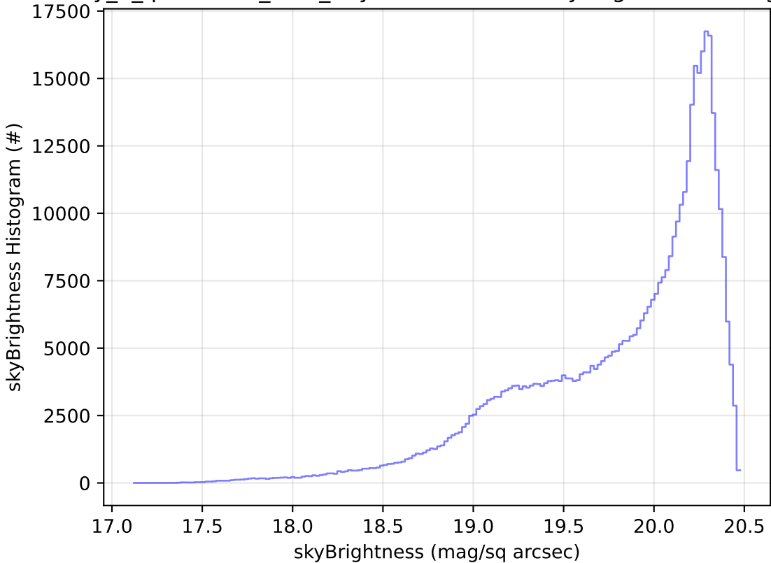
early_u_fpextra3.0_v3.4_10yrs WFD i band: skyBrightness Histogram
