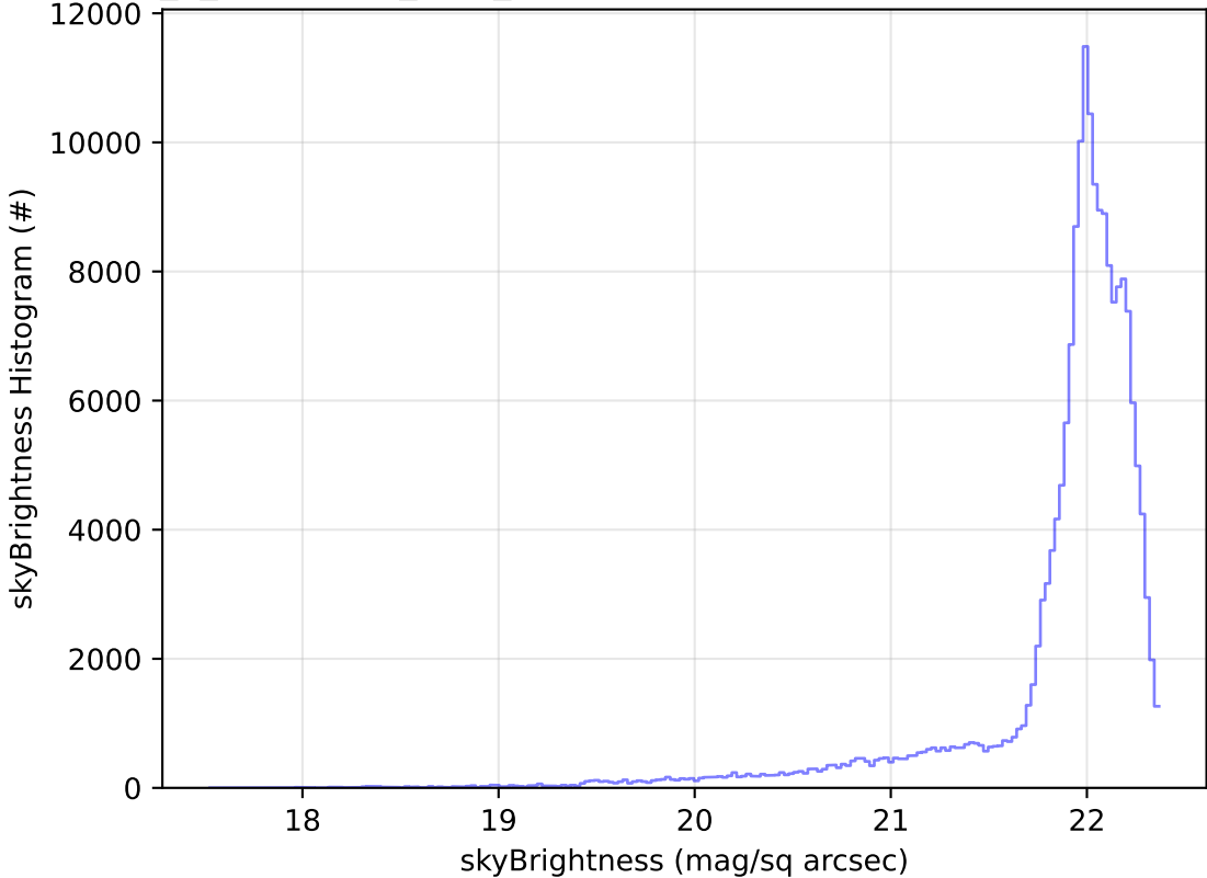
early_u_fpextra3.0_v3.4_10yrs WFD g band: skyBrightness Histogram
