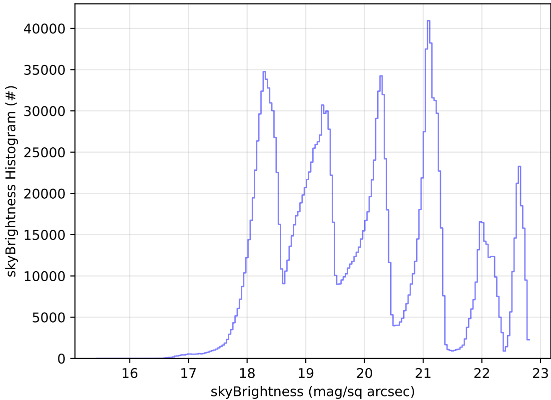
early_u_fpextra3.0_v3.4_10yrs WFD all bands: skyBrightness Histogram
