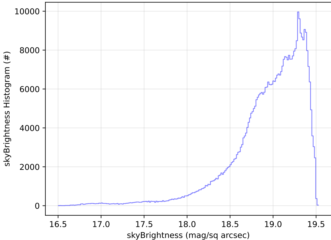
early_u_fpextra3.0_v3.4_10yrs All sky z band: skyBrightness Histogram
