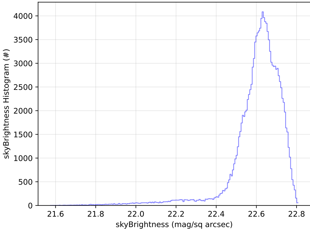
early_u_fpextra3.0_v3.4_10yrs All sky u band: skyBrightness Histogram
