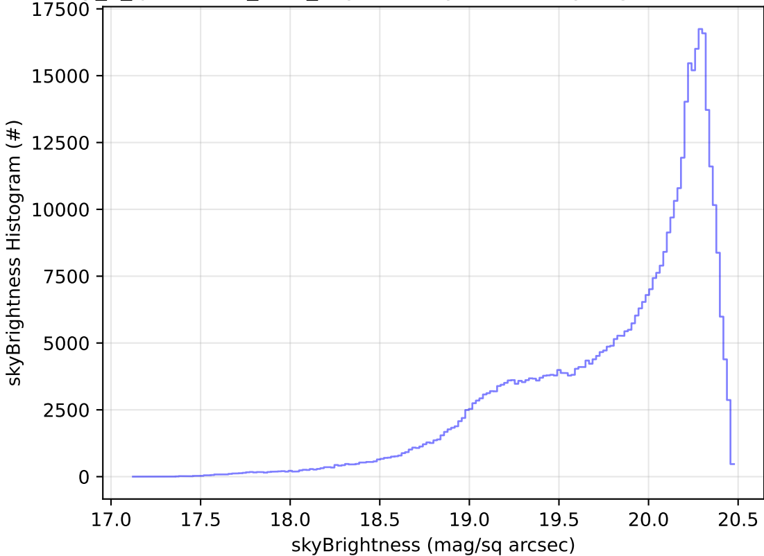
early_u_fpextra3.0_v3.4_10yrs All sky i band: skyBrightness Histogram
