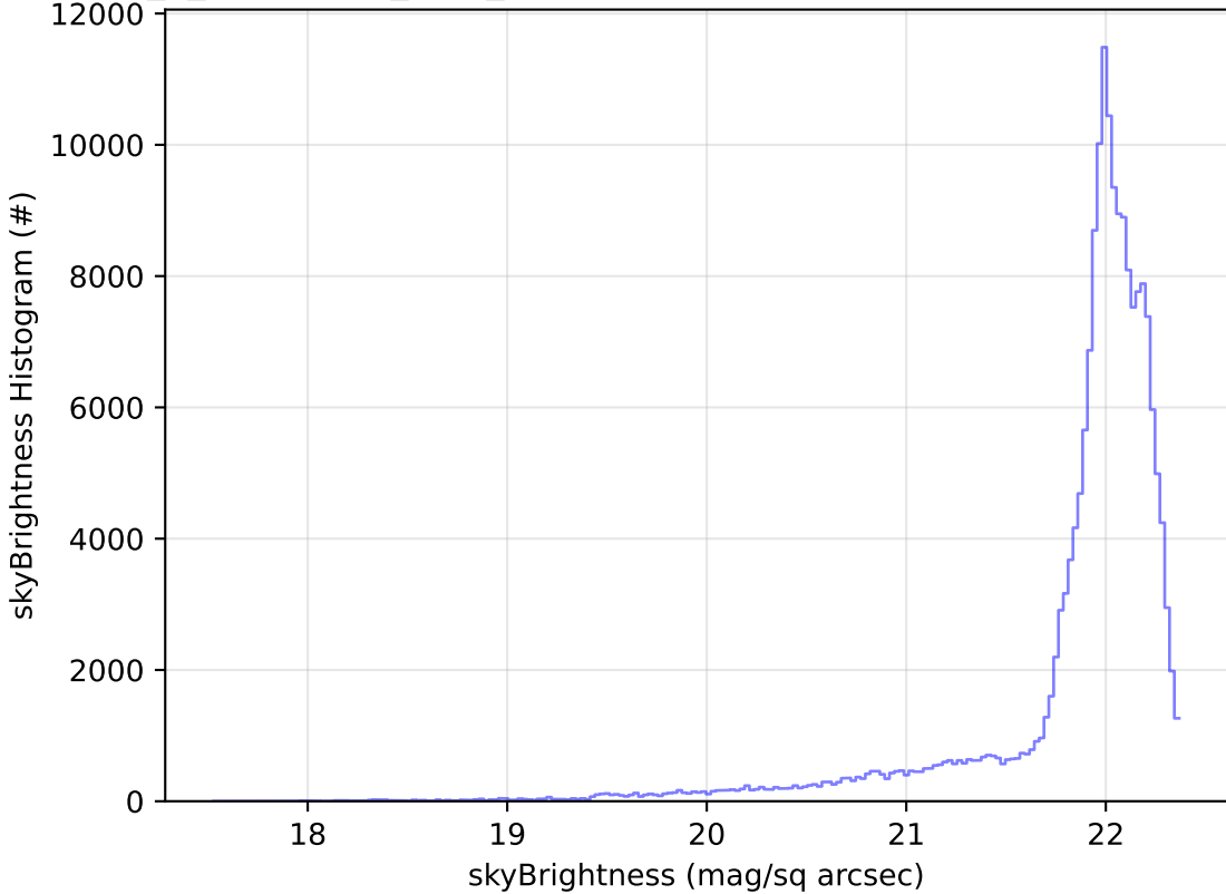
early_u_fpextra3.0_v3.4_10yrs All sky g band: skyBrightness Histogram
