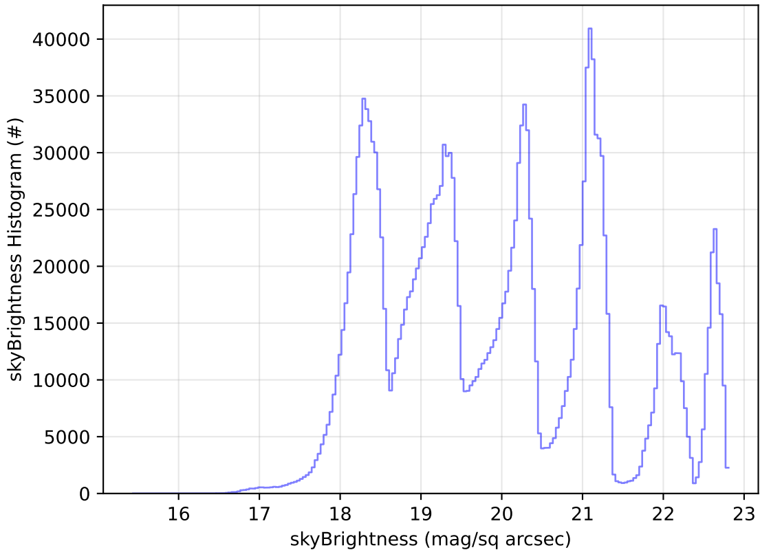
early_u_fpextra3.0_v3.4_10yrs All sky all bands: skyBrightness Histogram
