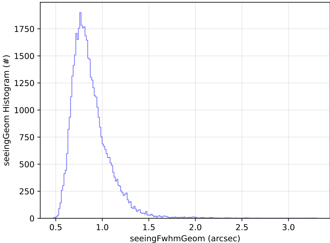
early_u_fpextra3.0_v3.4_10yrs Yr 1 y band: seeingGeom Histogram
