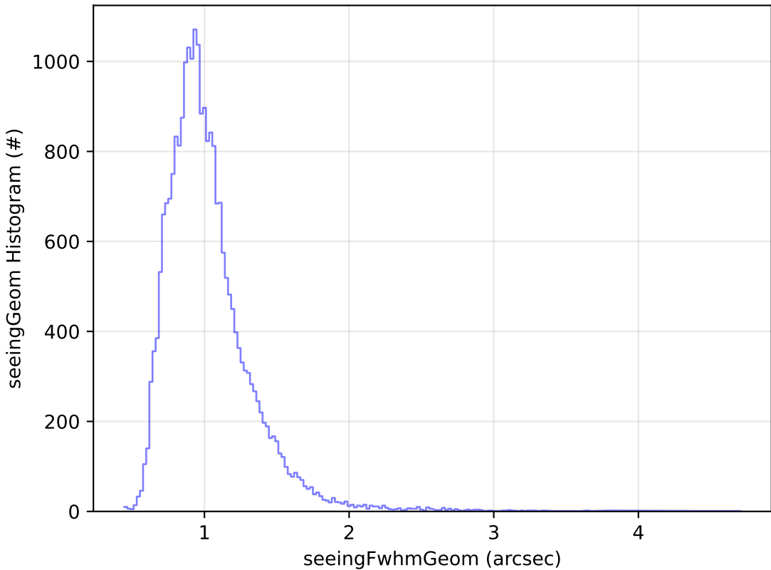
early_u_fpextra3.0_v3.4_10yrs Yr 1 u band: seeingGeom Histogram
