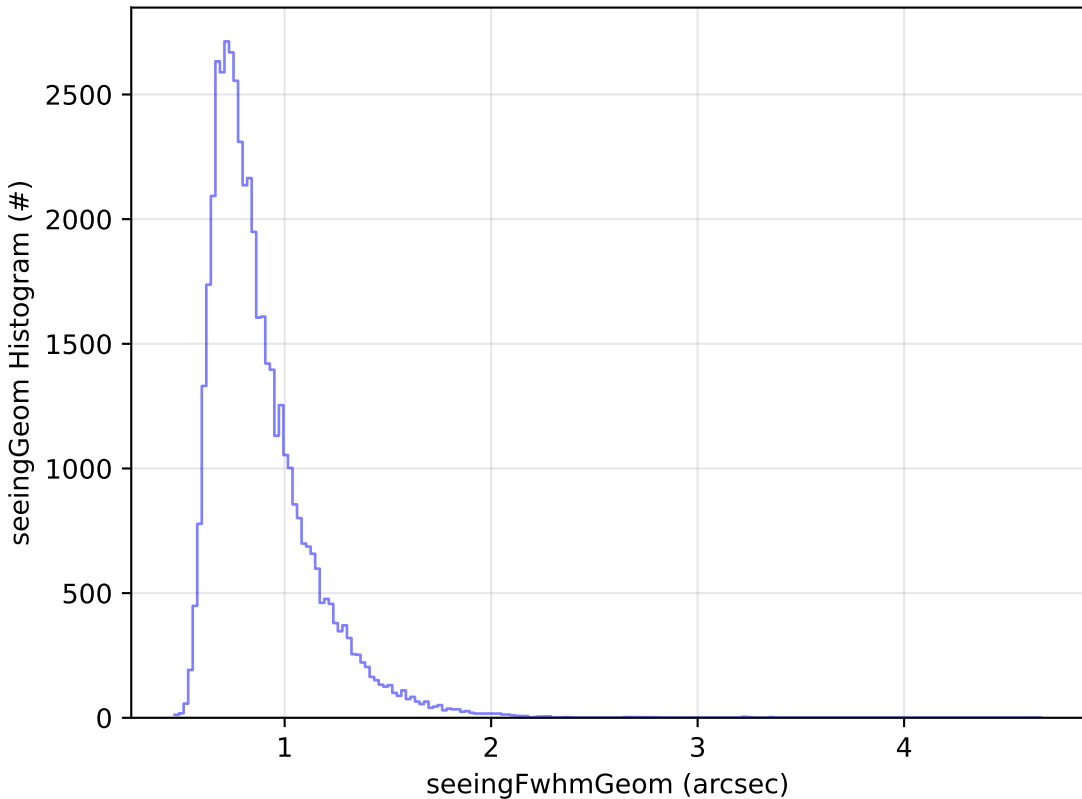
early_u_fpextra3.0_v3.4_10yrs Yr 1 r band: seeingGeom Histogram
