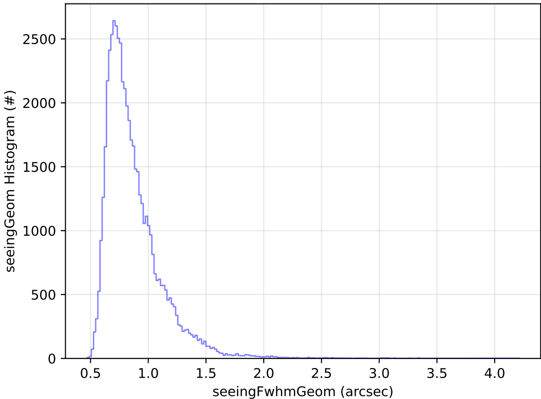
early_u_fpextra3.0_v3.4_10yrs Yr 1 i band: seeingGeom Histogram
