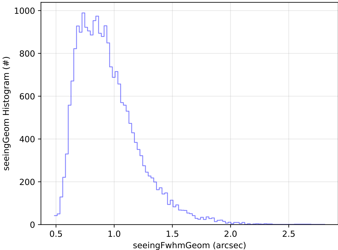
early_u_fpextra3.0_v3.4_10yrs Yr 1 g band: seeingGeom Histogram
