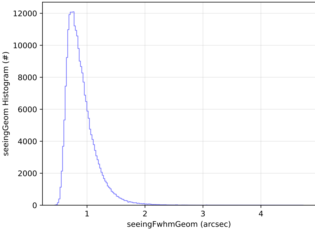
early_u_fpextra3.0_v3.4_10yrs Yr 1 all bands: seeingGeom Histogram
