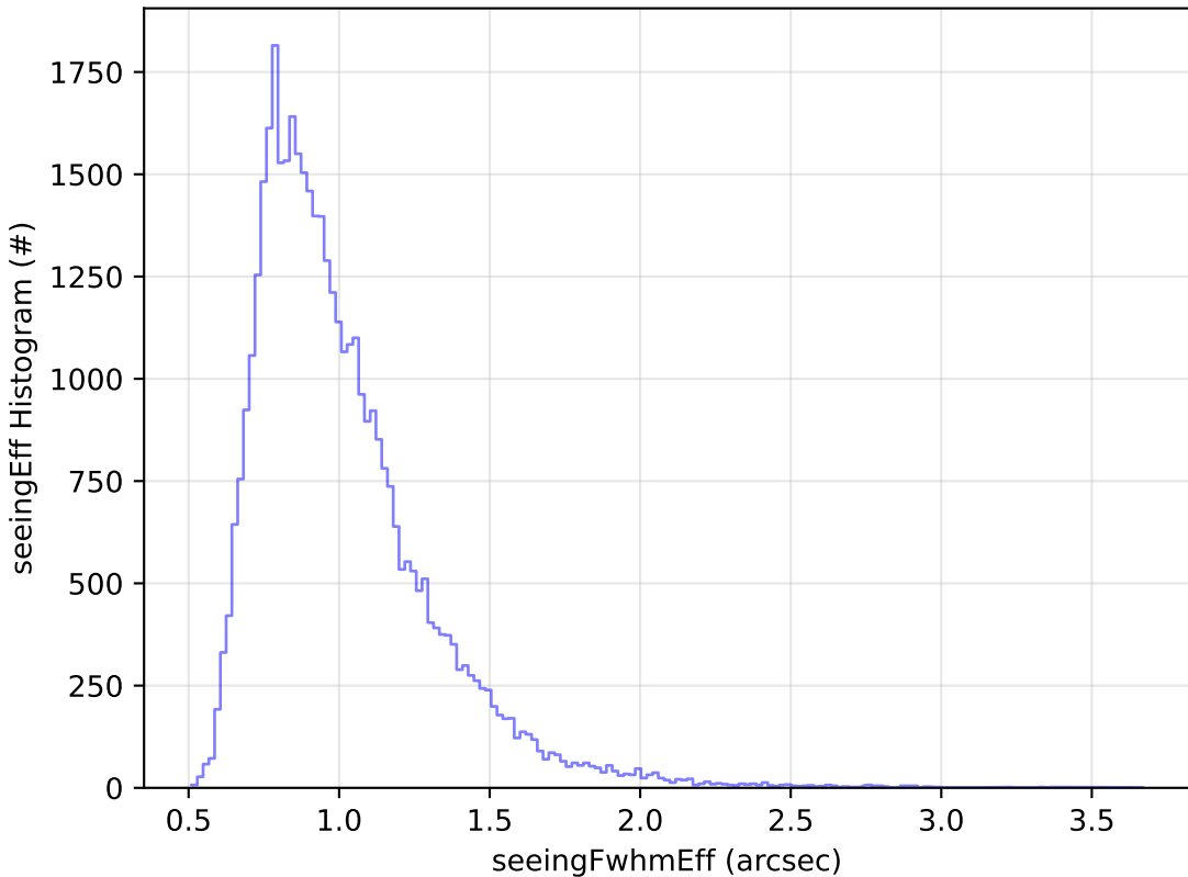
early_u_fpextra3.0_v3.4_10yrs Yr 1 z band: seeingEff Histogram
