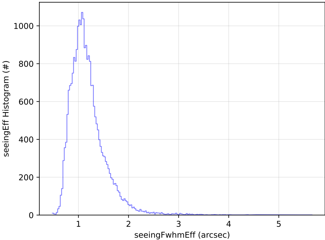
early_u_fpextra3.0_v3.4_10yrs Yr 1 u band: seeingEff Histogram
