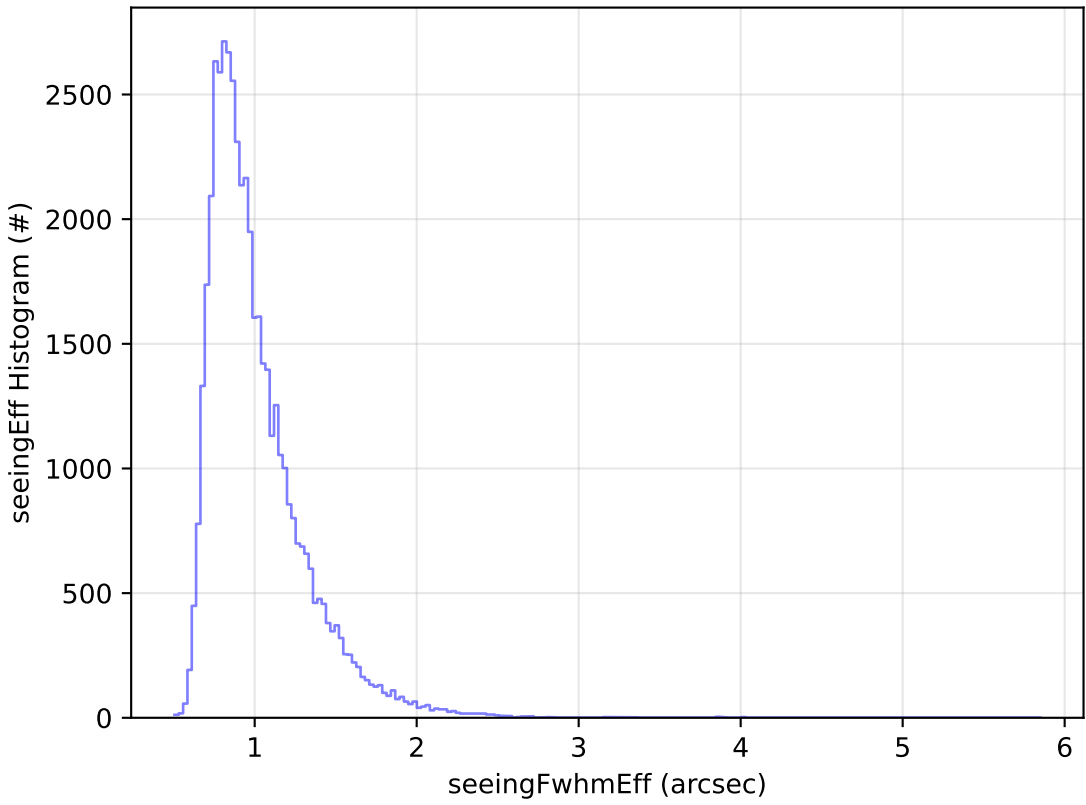
early_u_fpextra3.0_v3.4_10yrs Yr 1 r band: seeingEff Histogram
