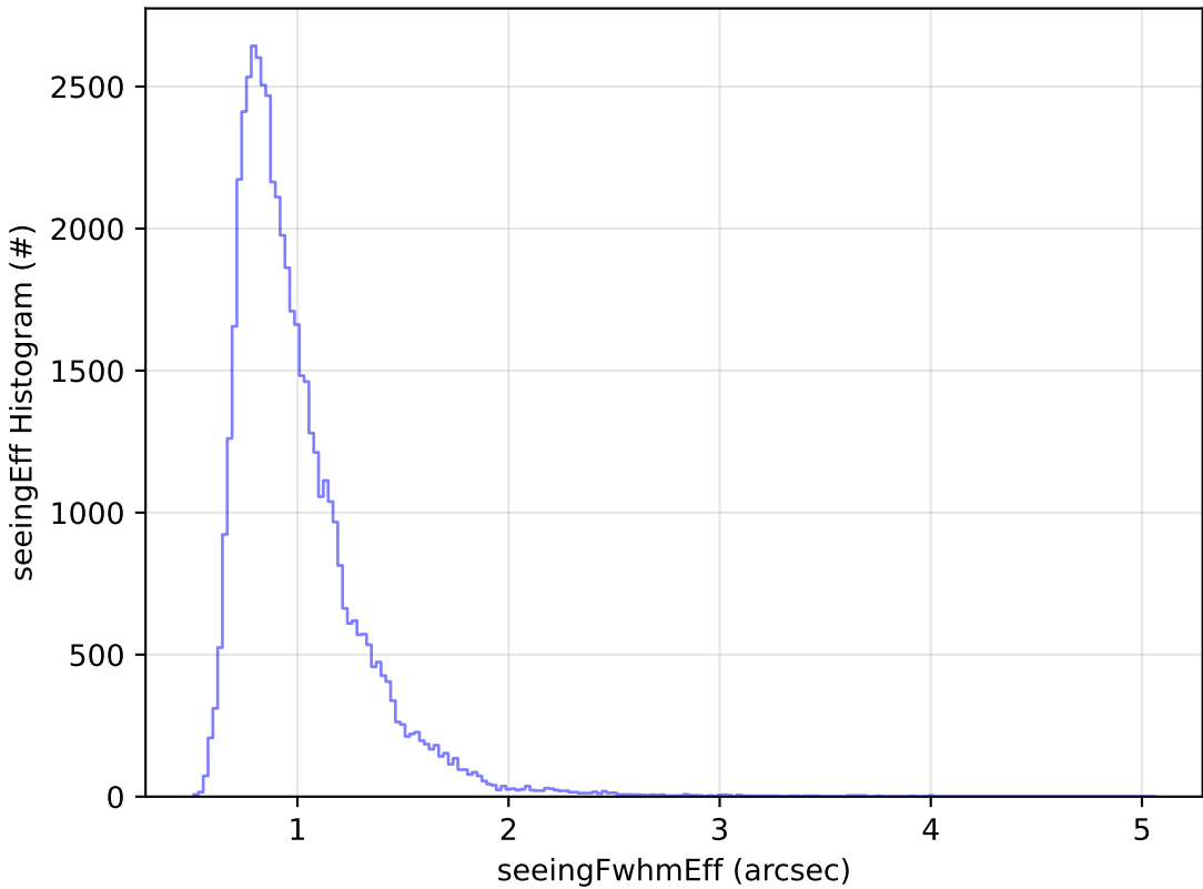
early_u_fpextra3.0_v3.4_10yrs Yr 1 i band: seeingEff Histogram
