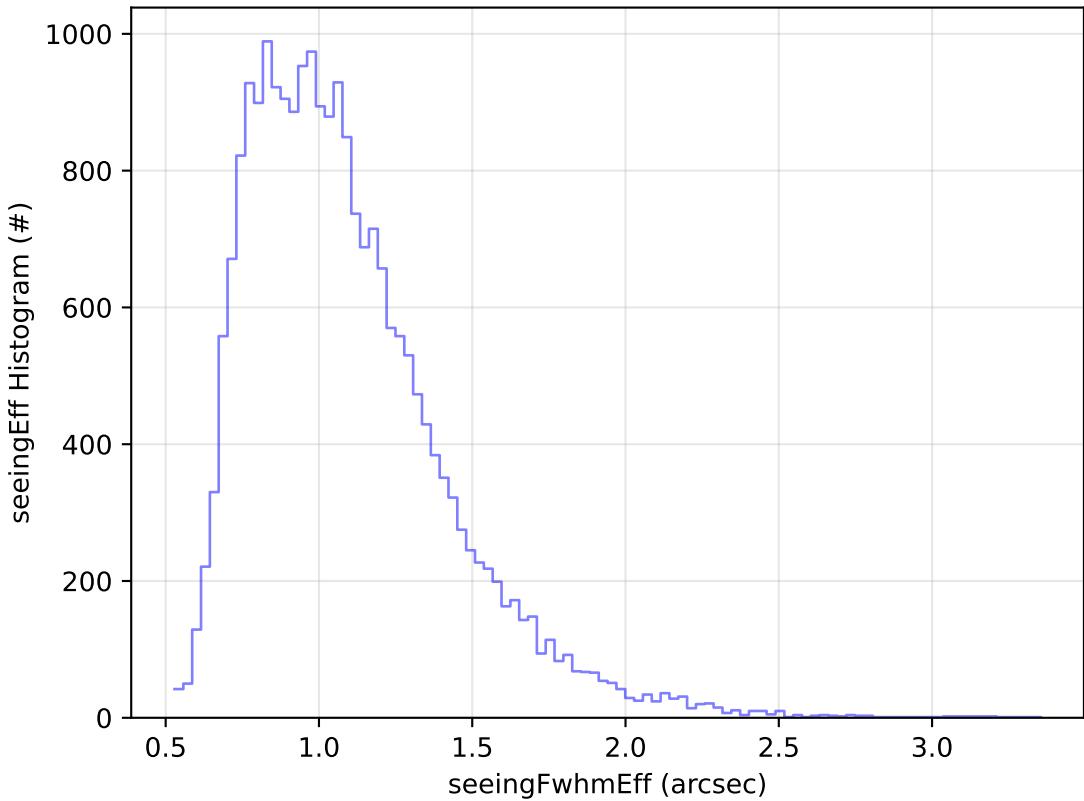
early_u_fpextra3.0_v3.4_10yrs Yr 1 g band: seeingEff Histogram
