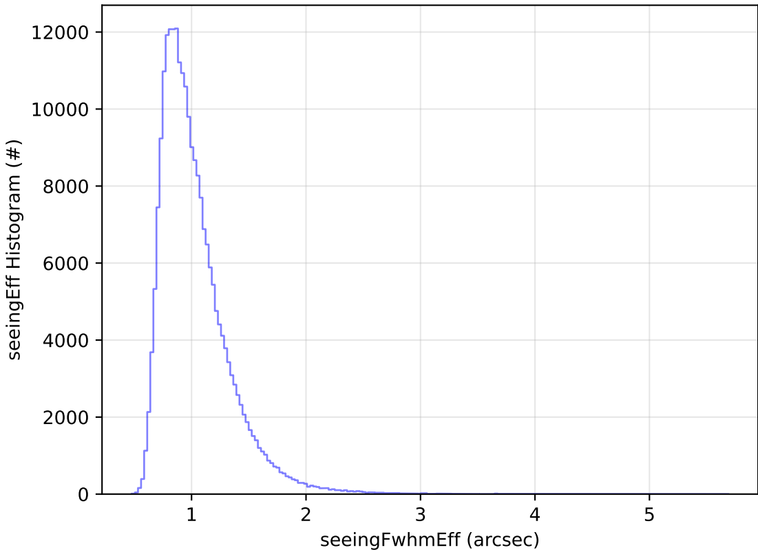
early_u_fpextra3.0_v3.4_10yrs Yr 1 all bands: seeingEff Histogram
