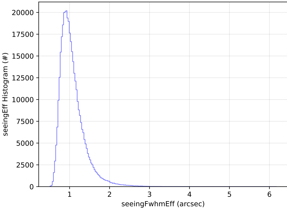
early_u_fpextra3.0_v3.4_10yrs WFD y band: seeingEff Histogram
