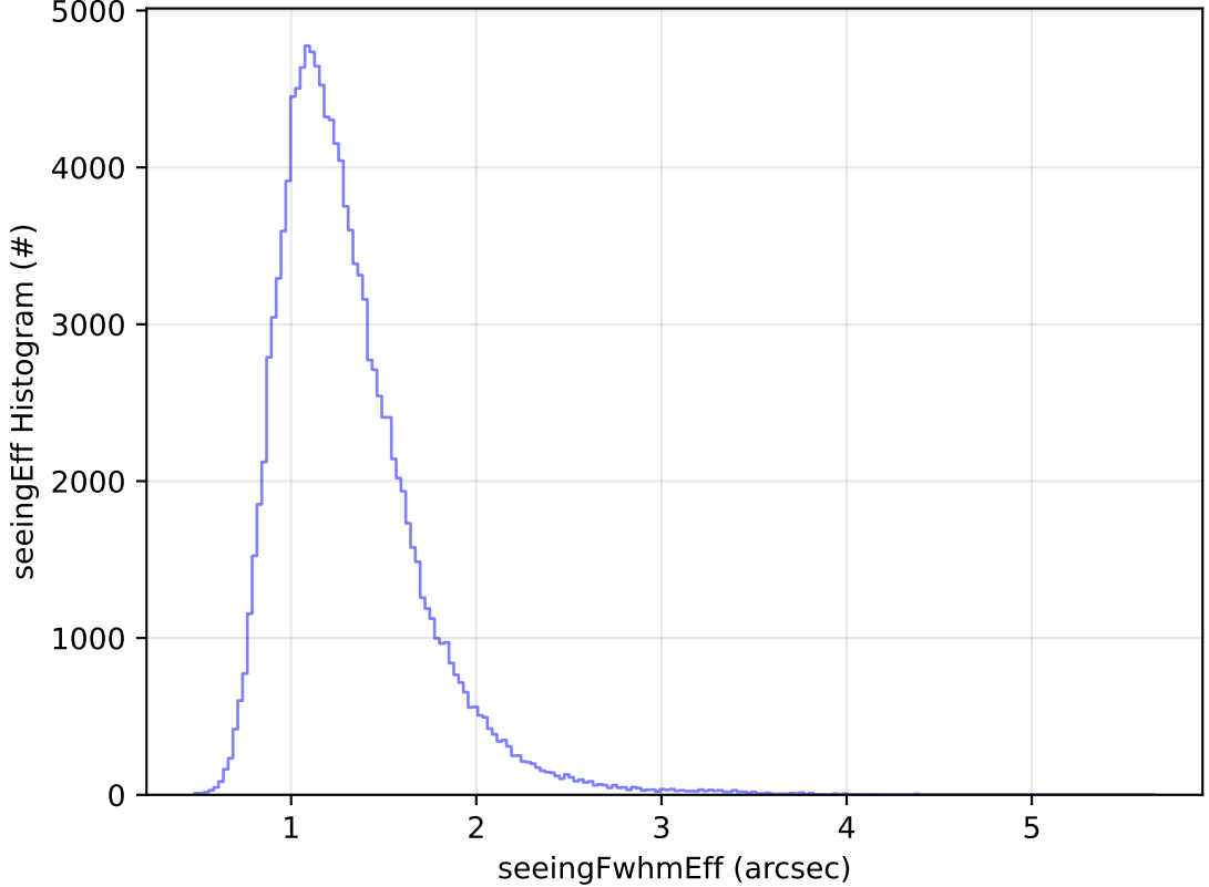
early_u_fpextra3.0_v3.4_10yrs WFD u band: seeingEff Histogram
