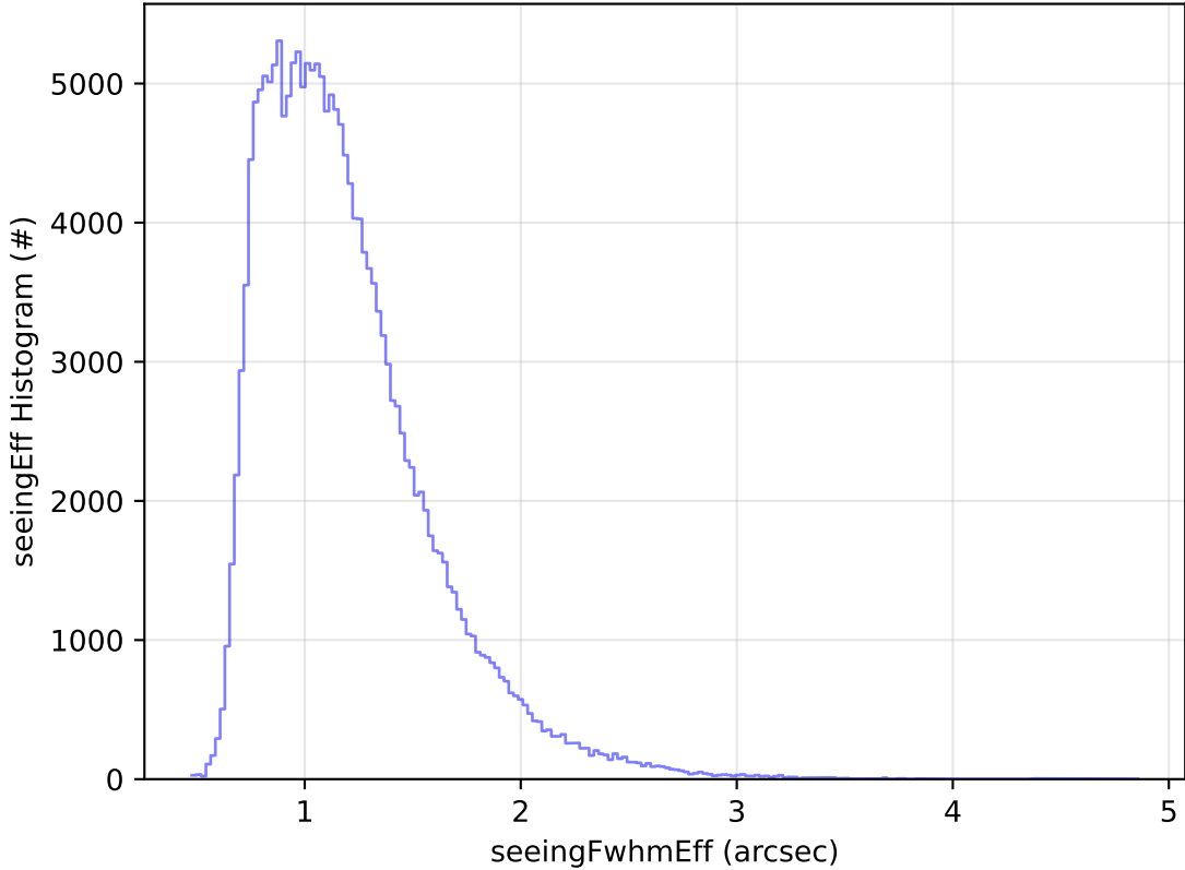
early_u_fpextra3.0_v3.4_10yrs WFD g band: seeingEff Histogram
