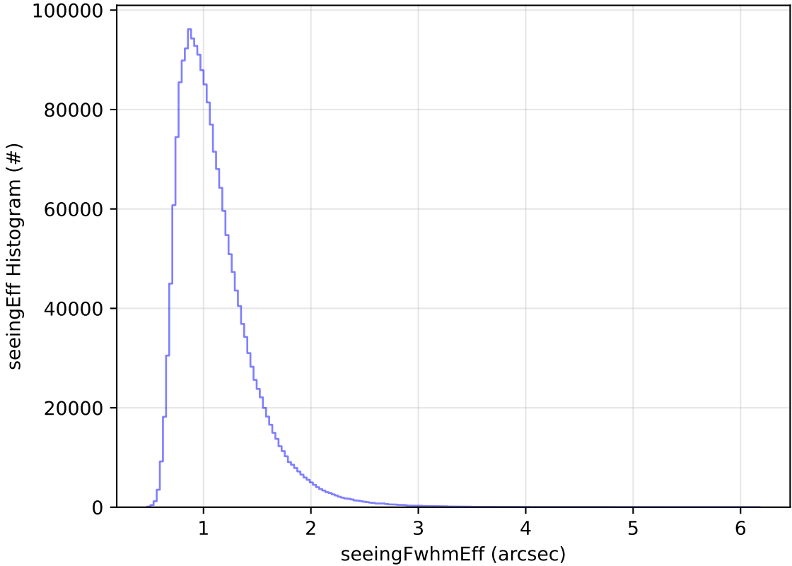
early_u_fpextra3.0_v3.4_10yrs WFD all bands: seeingEff Histogram
