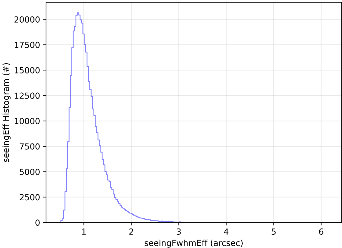
early_u_fpextra3.0_v3.4_10yrs All sky z band: seeingEff Histogram
