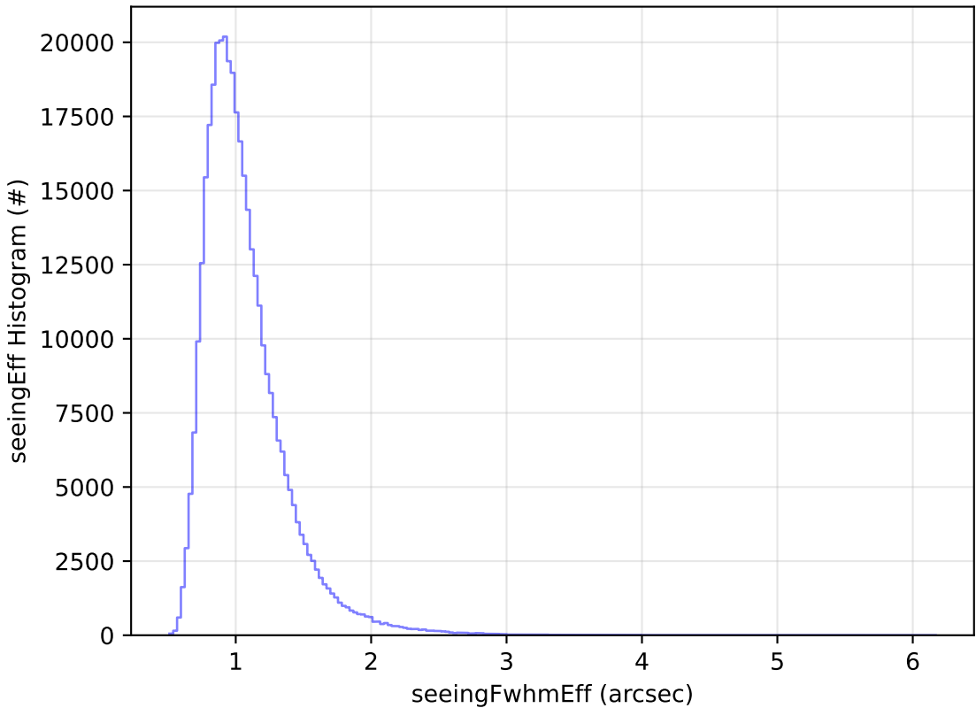
early_u_fpextra3.0_v3.4_10yrs All sky y band: seeingEff Histogram
