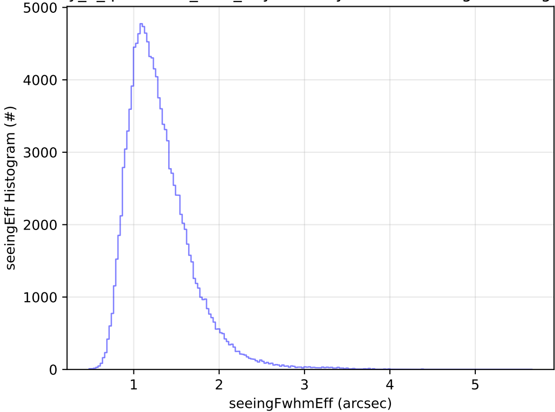
early_u_fpextra3.0_v3.4_10yrs All sky u band: seeingEff Histogram
