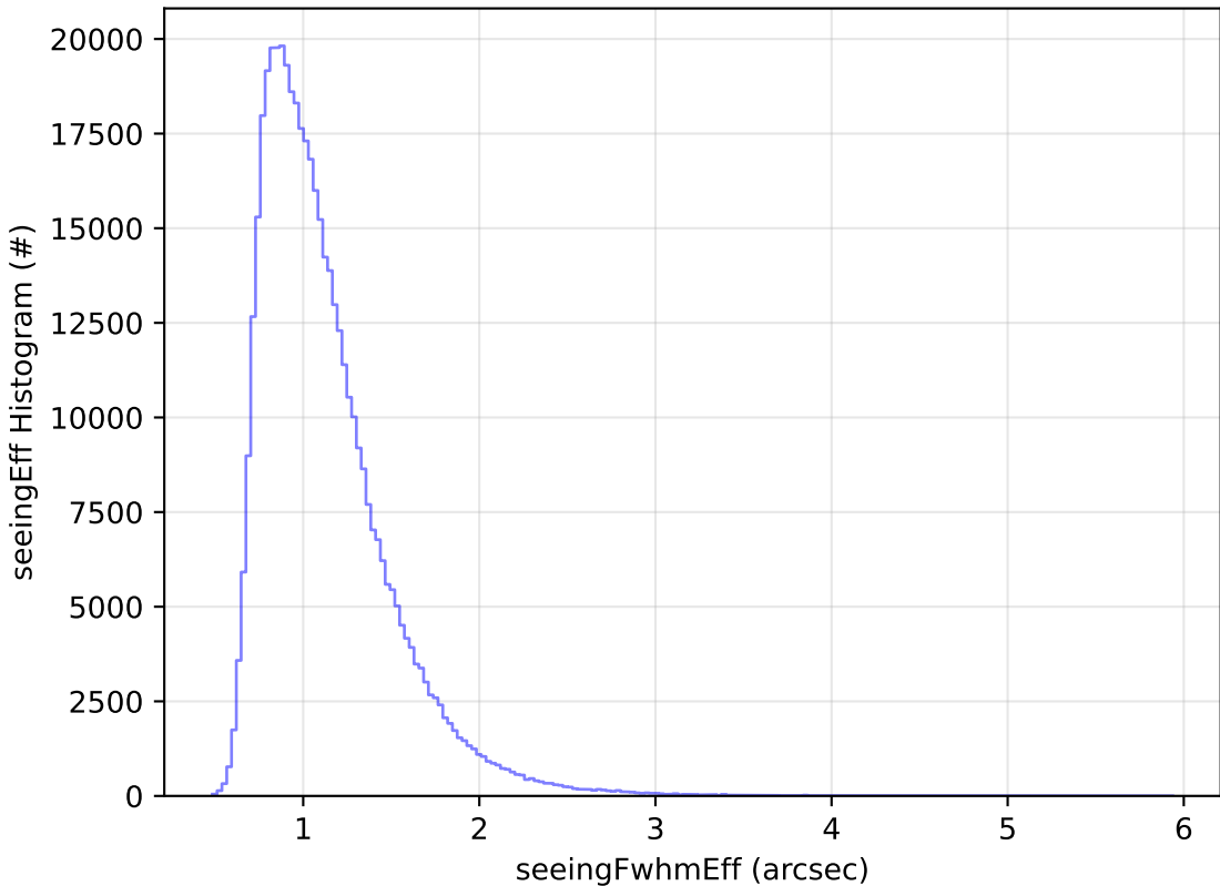
early_u_fpextra3.0_v3.4_10yrs All sky r band: seeingEff Histogram
