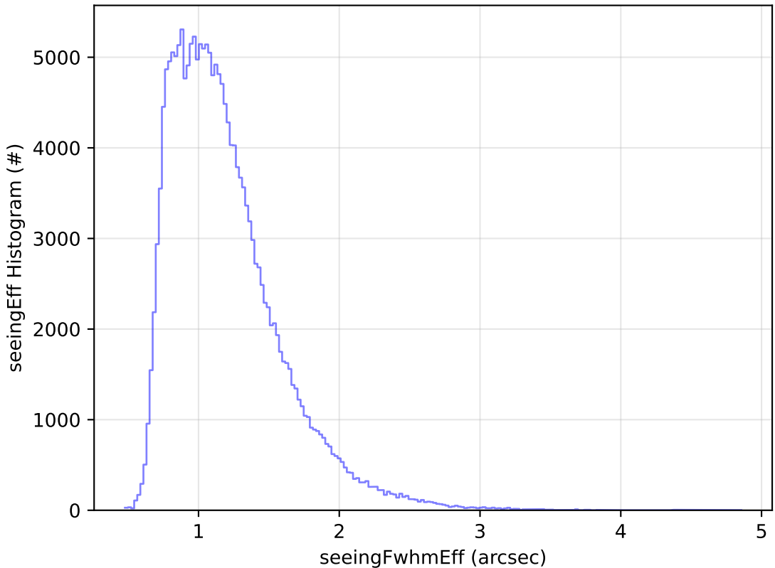
early_u_fpextra3.0_v3.4_10yrs All sky g band: seeingEff Histogram
