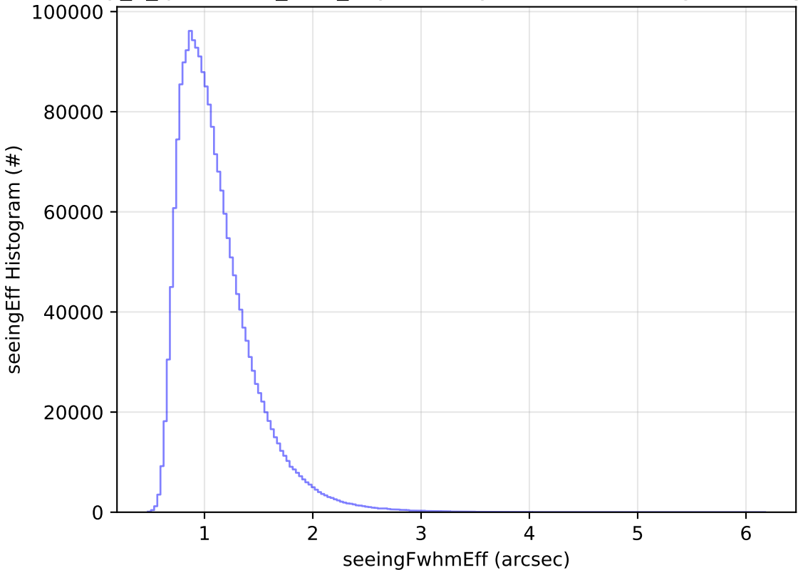
early_u_fpextra3.0_v3.4_10yrs All sky all bands: seeingEff Histogram
