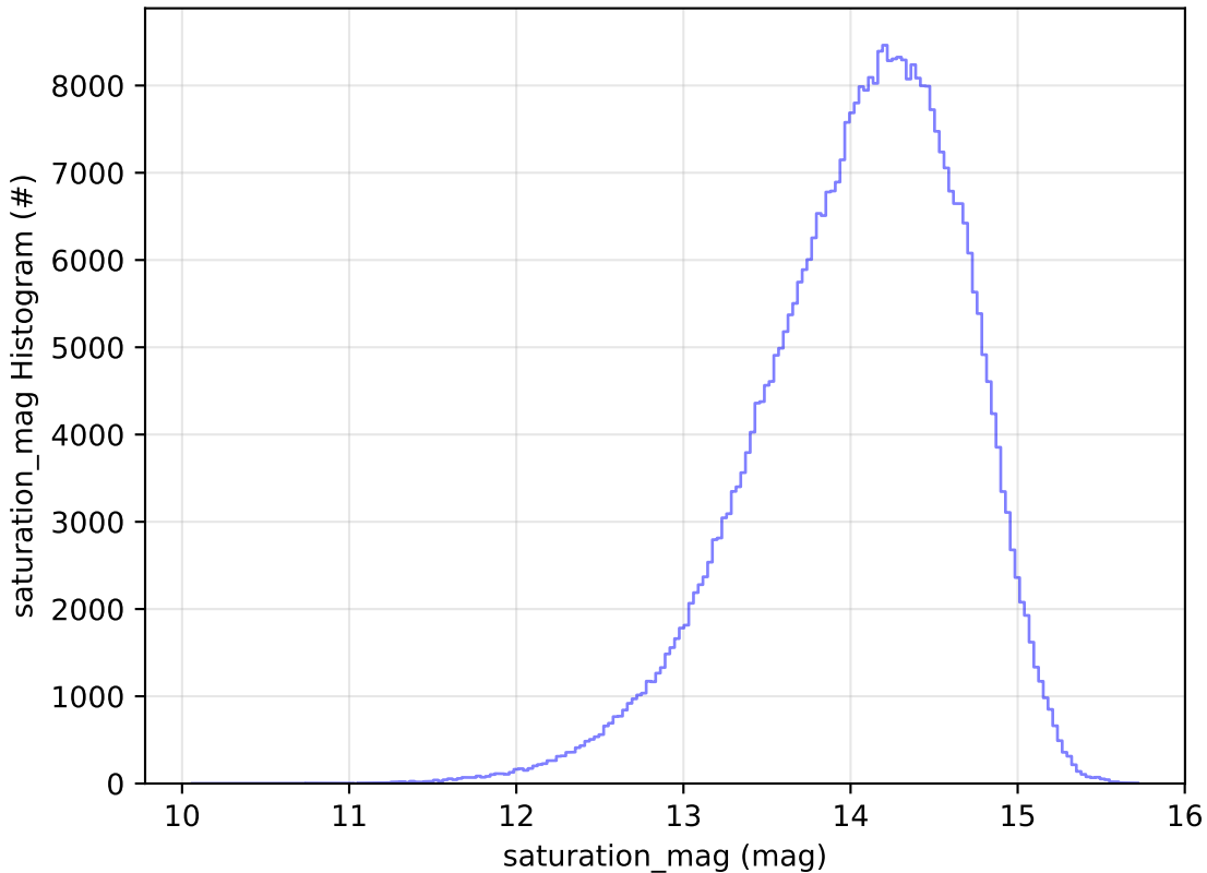
early_u_fpextra3.0_v3.4_10yrs WFD z band: saturation_mag Histogram
