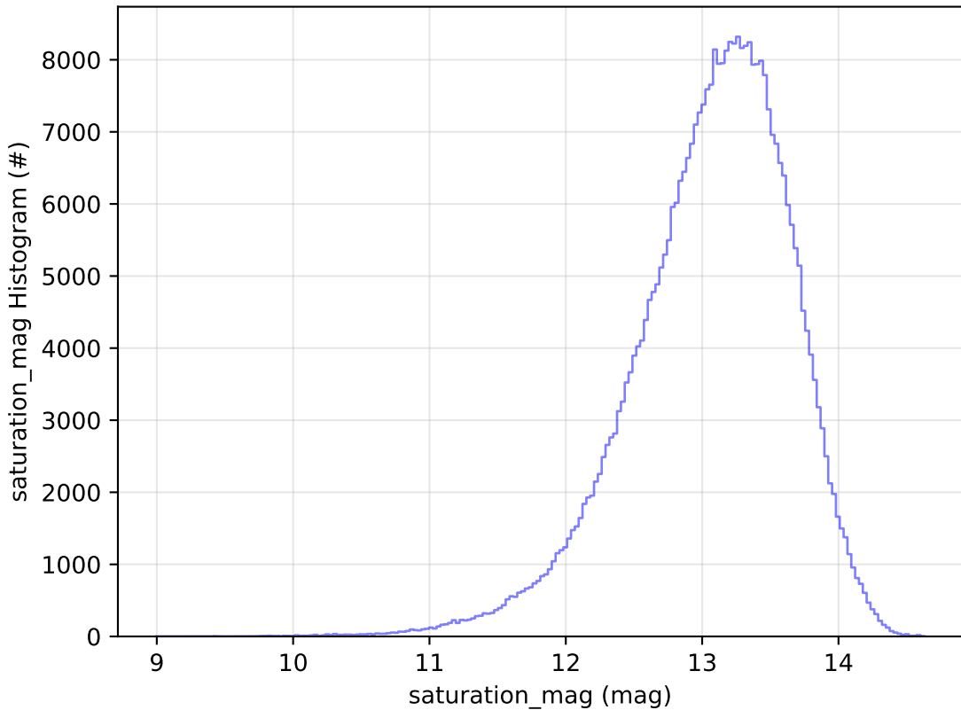
early_u_fpextra3.0_v3.4_10yrs WFD y band: saturation_mag Histogram
