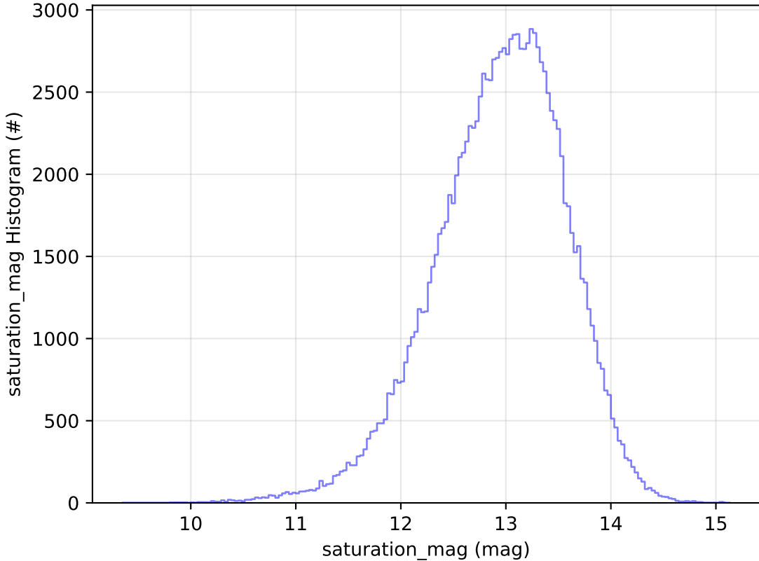
early_u_fpextra3.0_v3.4_10yrs WFD u band: saturation_mag Histogram
