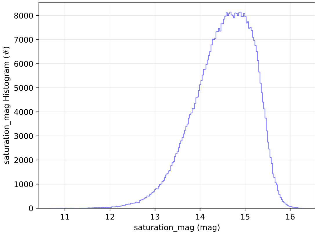
early_u_fpextra3.0_v3.4_10yrs WFD r band: saturation_mag Histogram
