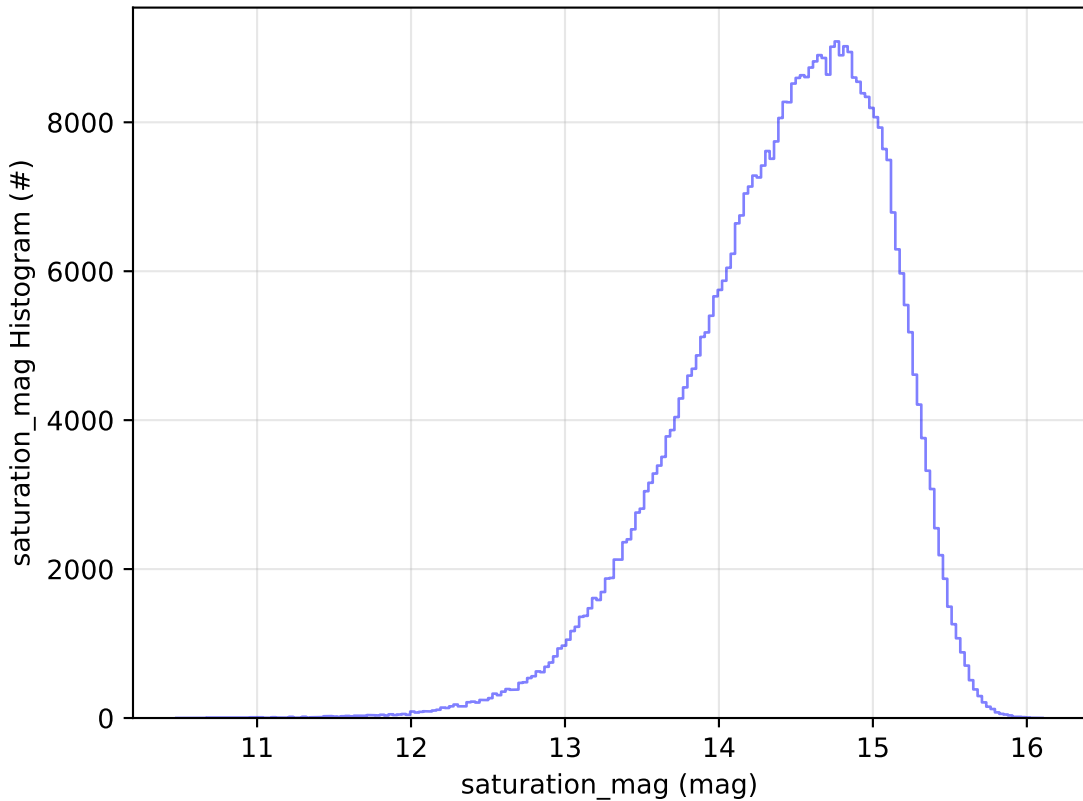
early_u_fpextra3.0_v3.4_10yrs WFD i band: saturation_mag Histogram
