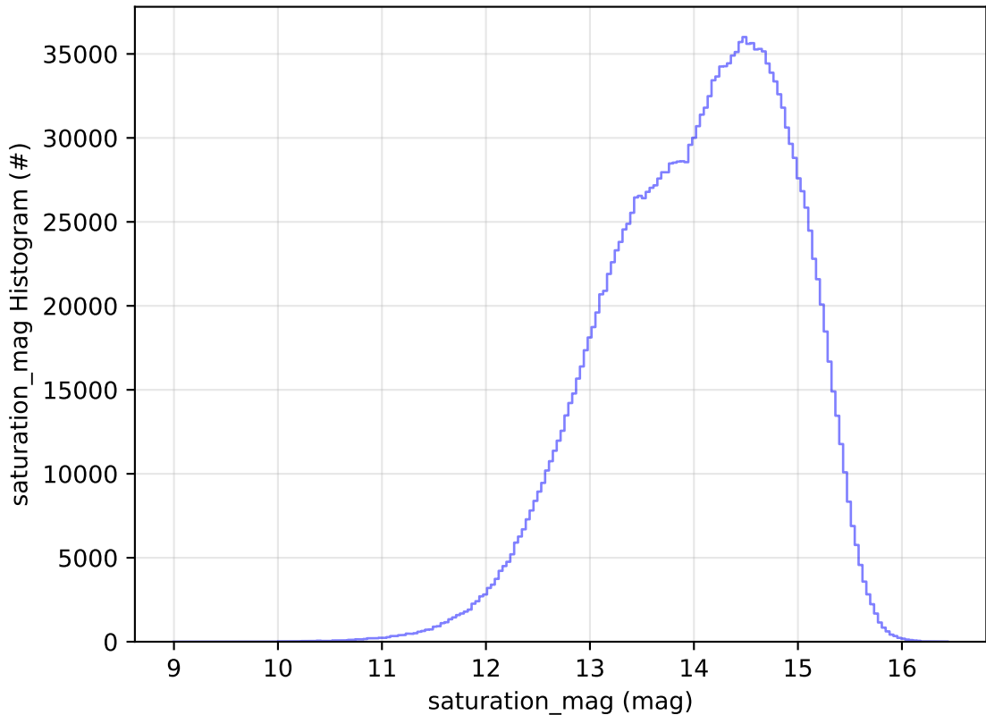
early_u_fpextra3.0_v3.4_10yrs WFD all bands: saturation_mag Histogram
