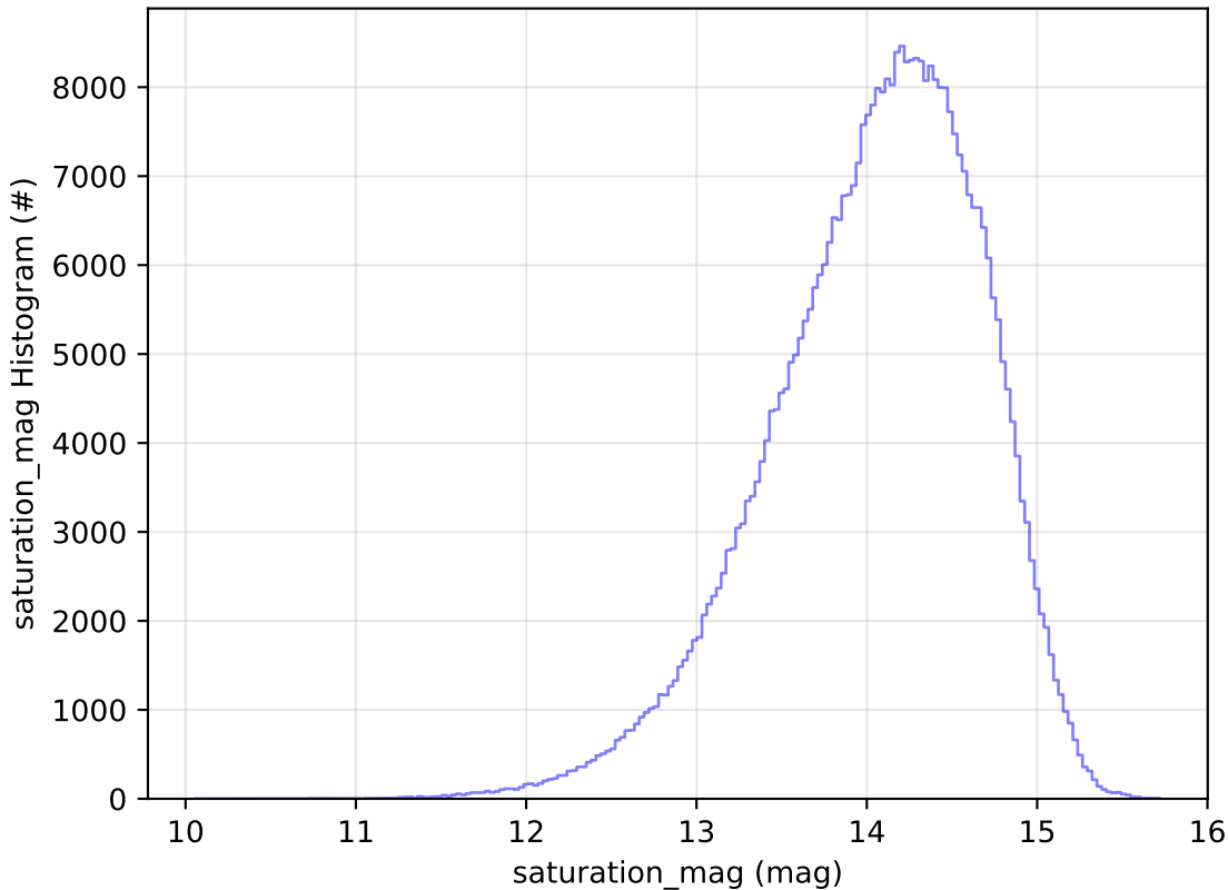
early_u_fpextra3.0_v3.4_10yrs All sky z band: saturation_mag Histogram
