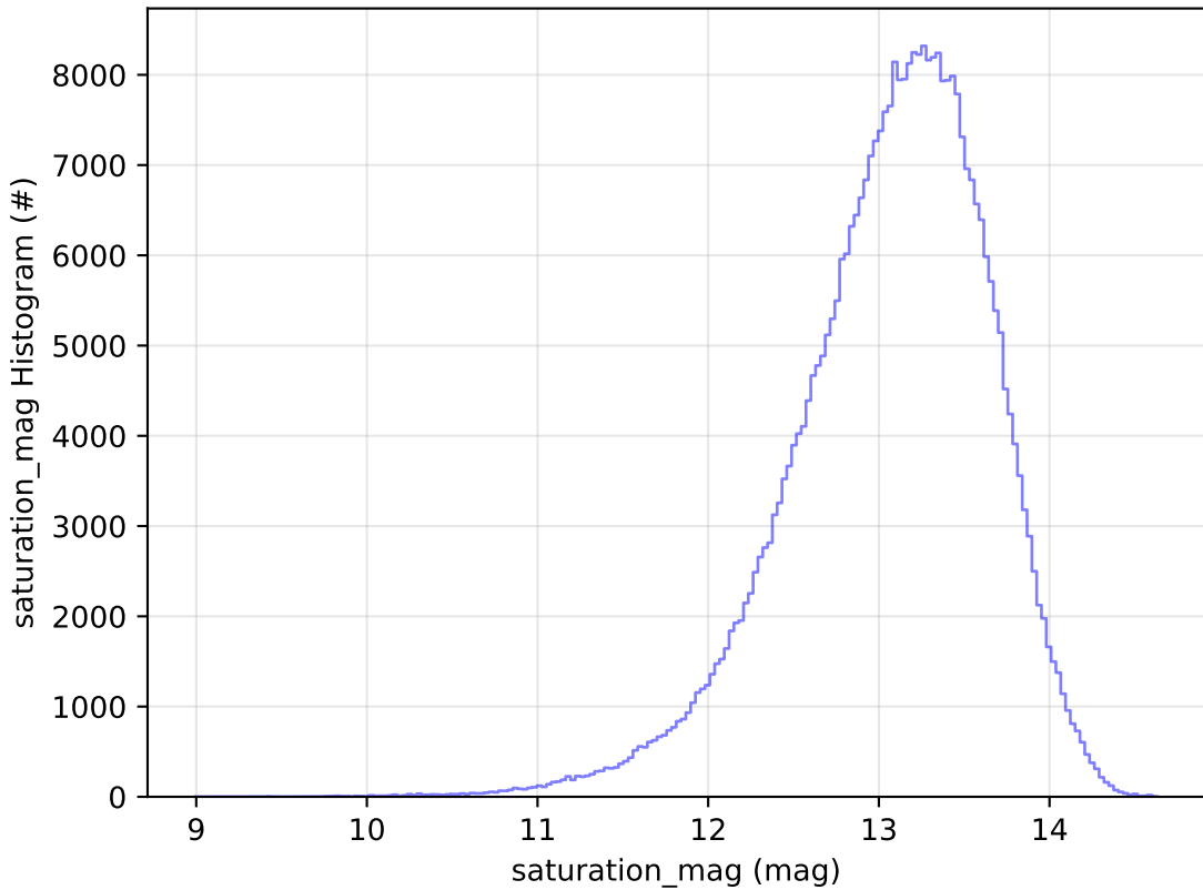
early_u_fpextra3.0_v3.4_10yrs All sky y band: saturation_mag Histogram
