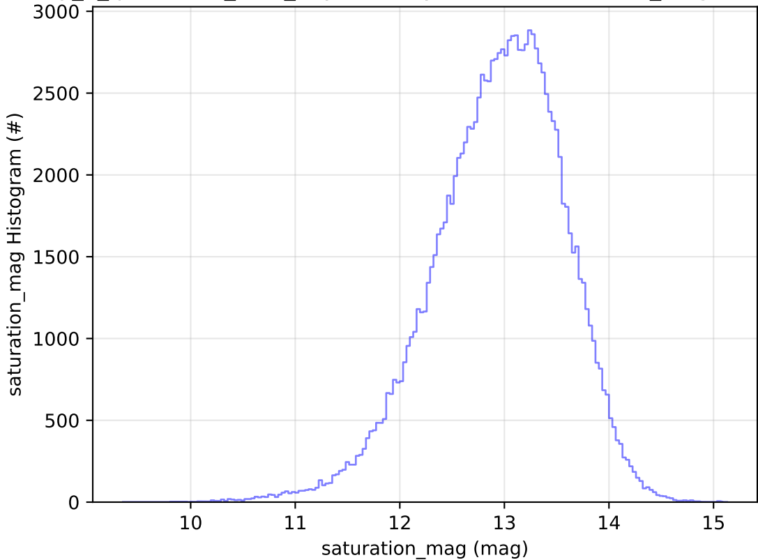
early_u_fpextra3.0_v3.4_10yrs All sky u band: saturation_mag Histogram
